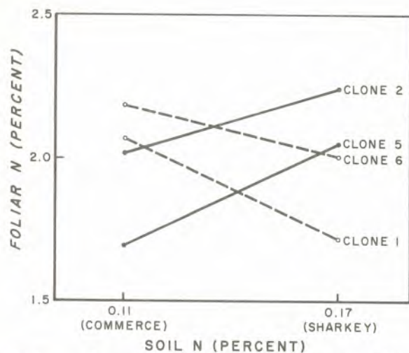
Figure 1.--Clonal X soil interaction for foliar N variation.
