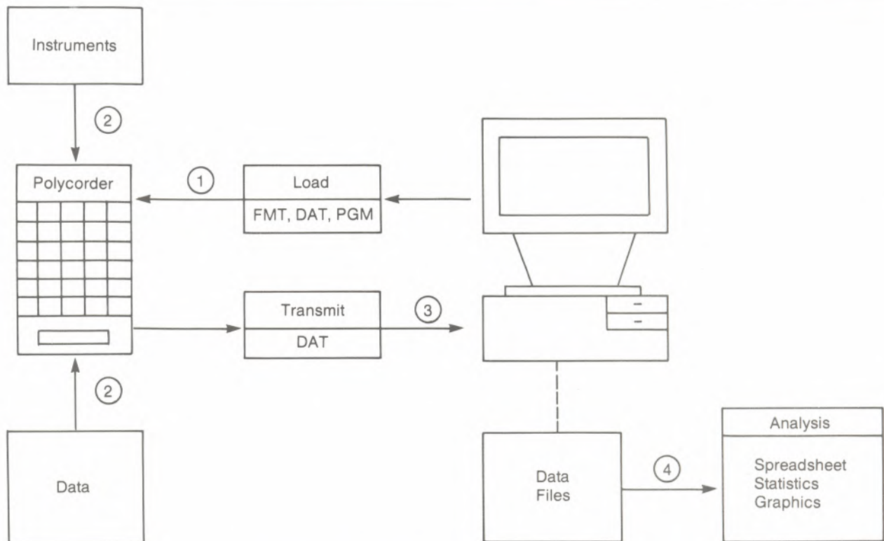
Figure 2—Typical scheme for collecting and processing research data with a portable data recorder.
