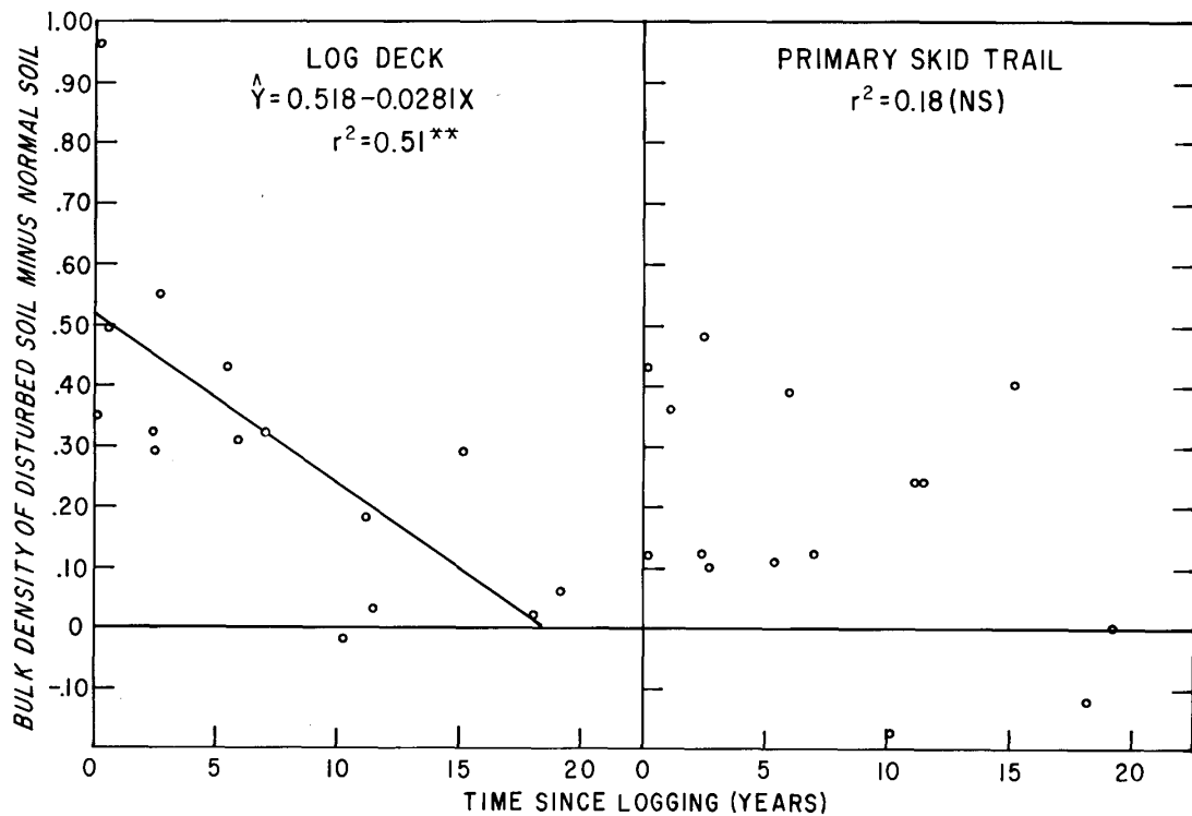
Figure 2.—Surface bulk density of disturbed soil minus normal soil density as related to time since logging.
