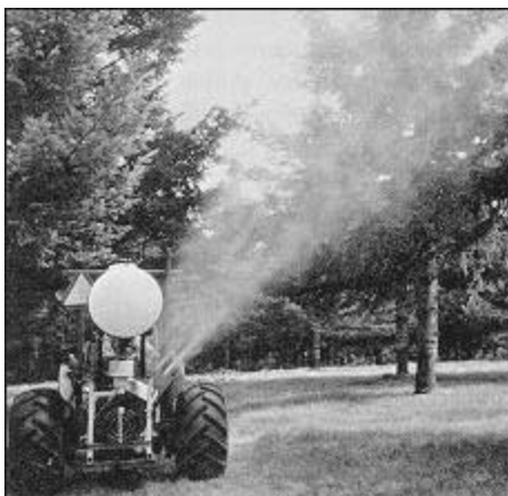
Figure 1. Wet pollen applicator.
