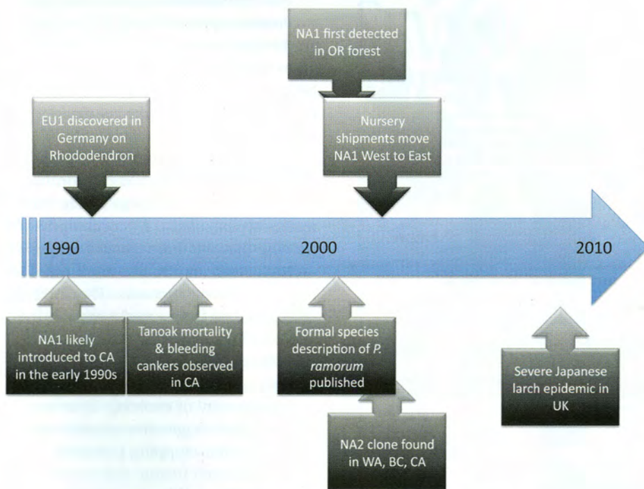
Figure 1: Chronology of the emergence of Phytophthora ramorum in North America
