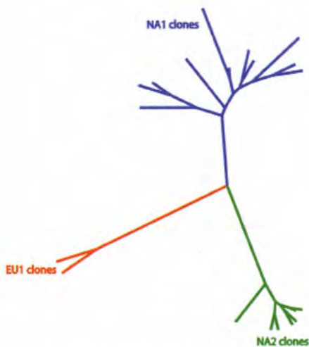
Figure 4: Research has shown that the three lineages of P. ramorum came from the same source but no longer interact with each other.
