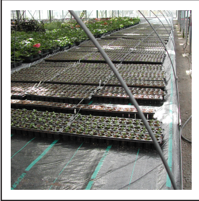
Figure 5. Using Aquamat with propagation trays.
