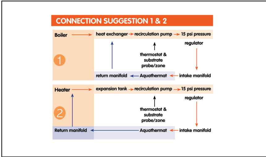
Figure 11. Connection suggestions for Aquathermat.
