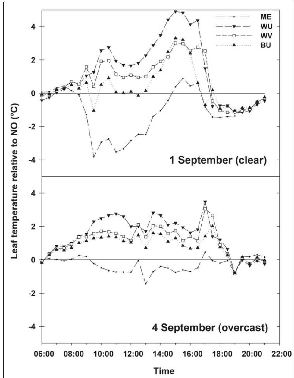
Figure 8—Leaf temperature (abaxial side of Oregon white oak seedling leaf) for seedlings (n = 2) in four tree shelter treatments, relative to leaf temperature of seedlings in ambient conditions (NO treatment; the 0 line) on a clear day with morning fog (1 September 2005) and on an overcast day (4 September 2005). Tree shelter treatments are a fine-mesh fabric shelter (ME), a solid-walled white unvented shelter (WU), a solid-walled white vented shelter (WV), and a solid-walled blue unvented shelter (BU).
