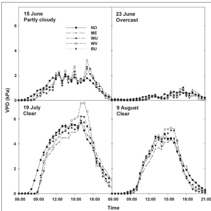
Figure 6—Vapor pressure deficit (VPD) in five tree shelter treatments on four days in 2005. Treatments are no tree shelter (NO), a fine-mesh fabric shelter (ME), a solid-walled white unvented shelter (WU), a solid-walled white vented shelter (WV), and a solid-walled blue unvented shelter (BU).
