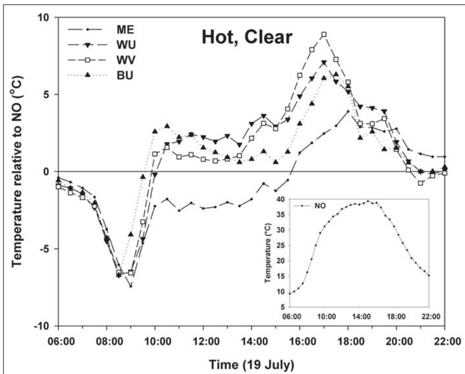
Figure 2—Air temperature in four tree shelter treatments, relative to no shelter, on 19 July 2005, a very hot, clear day. Inset graph shows air temperature with no shelter (ambient condition). Treatments are no tree shelter (NO; the 0 line in the large graph), a fine-mesh fabric shelter (ME), a solid-walled white unvented shelter (WU), a solid-walled white vented shelter (WV), and a solid-walled blue unvented shelter (BU).
