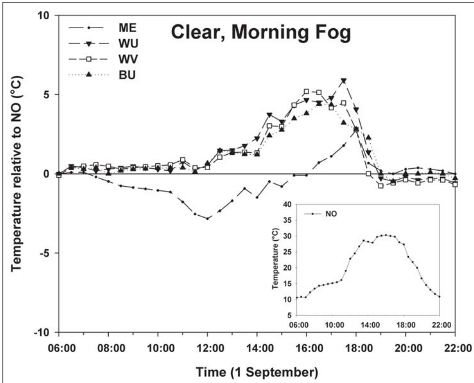
Figure 3—Air temperature in four tree shelter treatments, relative to no shelter, on 1 September 2005, a clear day with morning fog. Inset graph shows air temperature with no shelter (ambient condition). Treatments are no tree shelter (NO; the 0 line in the large graph), a fine-mesh fabric shelter (ME), a solid-walled white unvented shelter (WU), a solid-walled white vented shelter (WV), and a solid-walled blue unvented shelter (BU).
