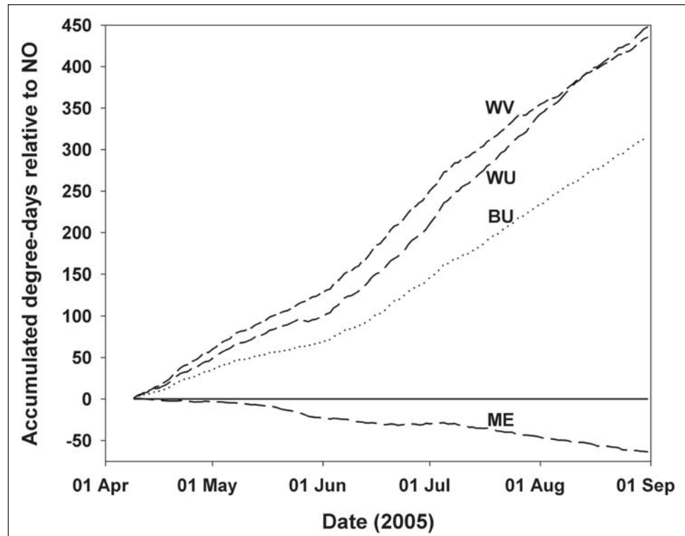
Figure 5—Accumulated degree days (base temperature = 5.0 °C) relative to ambient conditions (NO treatment; the 0 line) during the 2005 growing season for four tree shelter treatments. Treatments are a fine-mesh fabric shelter (ME), a solid-walled white unvented shelter (WU), a solid-walled white vented shelter (WV), and a solid-walled blue unvented shelter (BU).
