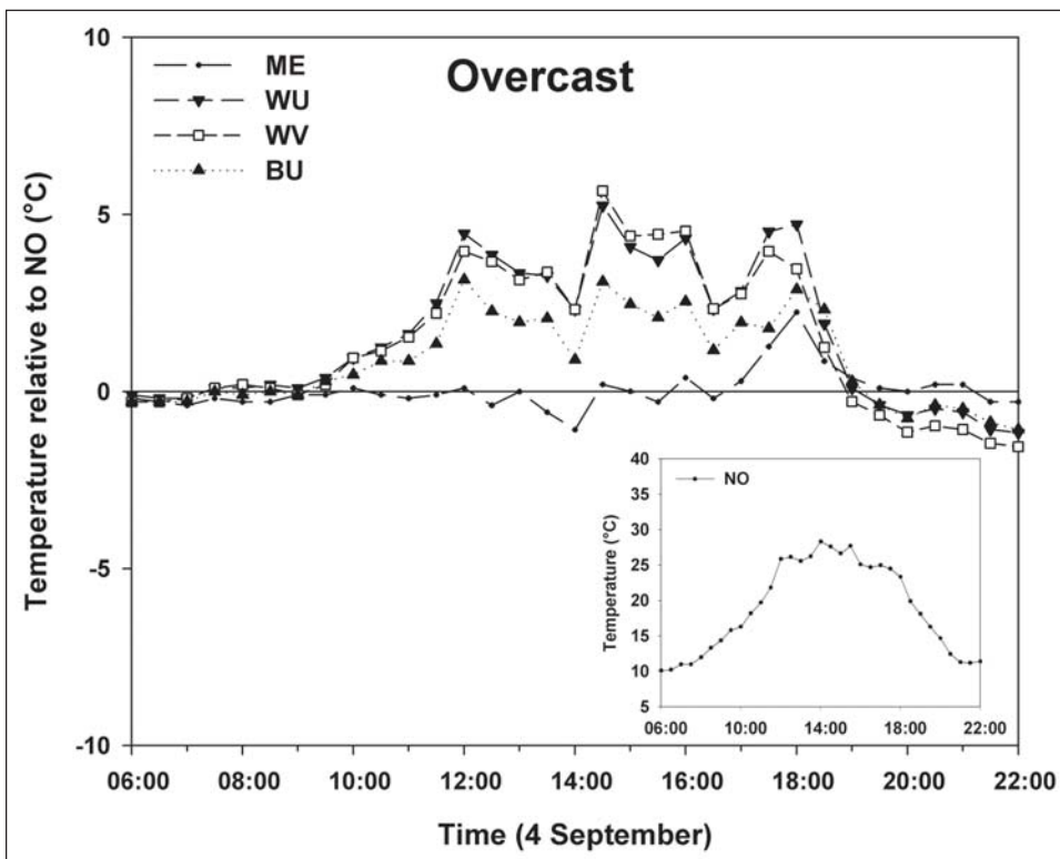
Figure 4—Air temperature in four tree shelter treatments, relative to no shelter, on 4 September 2005, an overcast day. Inset graph shows air temperature with no shelter (ambient condition). Treatments are no tree shelter (NO; the 0 line in the large graph), a fine-mesh fabric shelter (ME), a solid-walled white unvented shelter (WU), a solid-walled white vented shelter (WV), and a solid-walled blue unvented shelter (BU).
