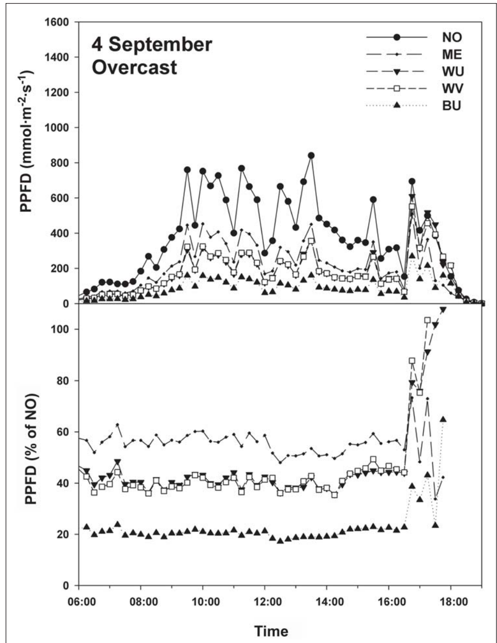
Figure 10—Photosynthetic photon flux density (PPFD) in five tree shelter treatments and PPFD relative to ambient conditions (NO treatment) on 4 September 2005, an overcast day. Treatments are no tree shelter (NO), a fine-mesh fabric shelter (ME), a solid-walled white unvented shelter (WU), a solid-walled white vented shelter (WV), and a solid-walled blue unvented shelter (BU).
