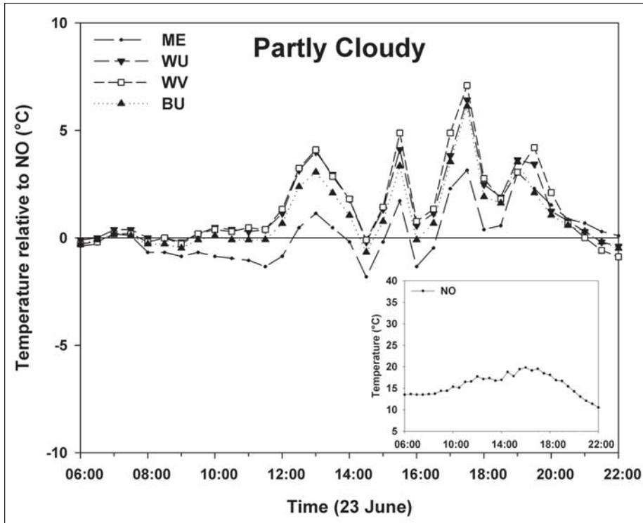
Figure 1—Air temperature in four tree shelter treatments, relative to no shelter, on 23 June 2005, a typical, partly cloudy day. Inset graph shows air temperature with no shelter (ambient condition). Treatments are no tree shelter (NO; the 0 line in the large graph), a fine-mesh fabric shelter (ME), a solid-walled white unvented shelter (WU), a solid-walled white vented shelter (WV), and a solid-walled blue unvented shelter (BU).
