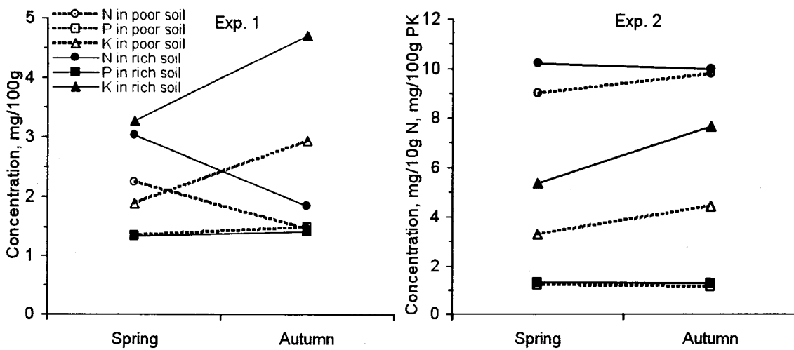
Fig 1. Means of soluble soil nitrogen and exchangeable phosphorus and potassium (N, P, K) during the first growing season of 2001 and 2002 in experiments 1 (n = 4 blocks) and 2 (n = 5 blocks).
