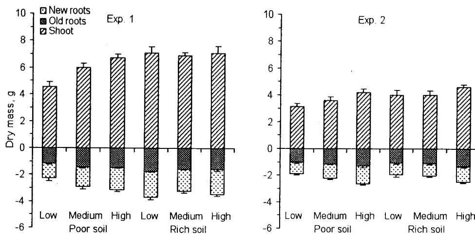
Fig 3. Seedling dry masses of shoot, new roots (root egress) and old roots after the first growing season in experiments 1 (n = 4 blocks) and 2 (n = 5 blocks) (mean+se).
