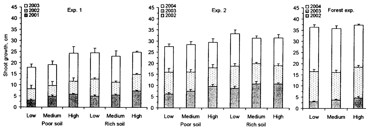
Fig 4. Yearly seedling height growth in experiments 1 (n = 4 blocks) and 2 (n = 5 blocks) and in the forest site experiment (n = 8 blocks) (mean + se).
