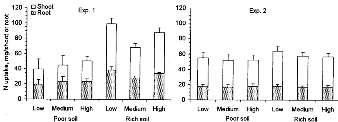
Fig 2. Uptake of nitrogen in the seedlings during the first growing season of 2001 and 2002 in the experiments 1 (n = 4 blocks) and 2 (n = 5 blocks) (mean+se). The initial nutrient contents have been assumed to be equal within the loading treatments.
