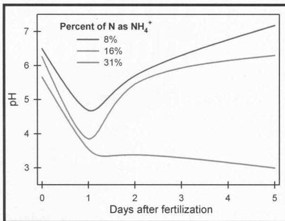
Figure 2. Change in pH of the root-zone of rose plants provided with three different percentages of ammonium. Plants were grown hydroponically, so pH fluctuations occurred much more rapidly than in a commercial growing medium, which is buffered by limestone additions.
