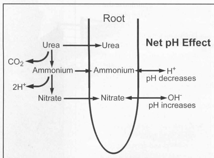
Figure 1. Conversions between nitrogen form and the effect of nitrogen uptake on growing medium pH.
