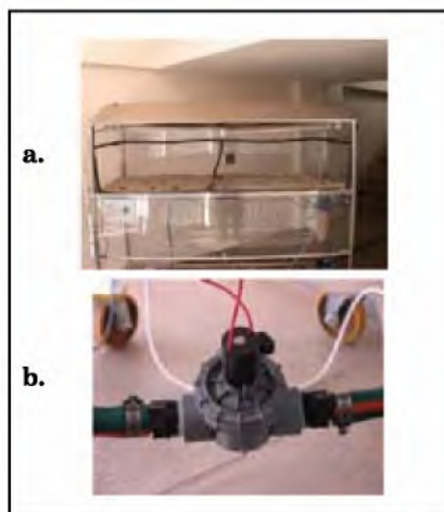
Figure 2. Wheelie Green 2 with PVC irrigation system attached to the chamber sides (a). The system has four non-drip mist spray nozzles. Normal municipal tap water pressure is adequate to open the nozzles. Irrigation is controlled by a solenoid valve on a timer (b).
