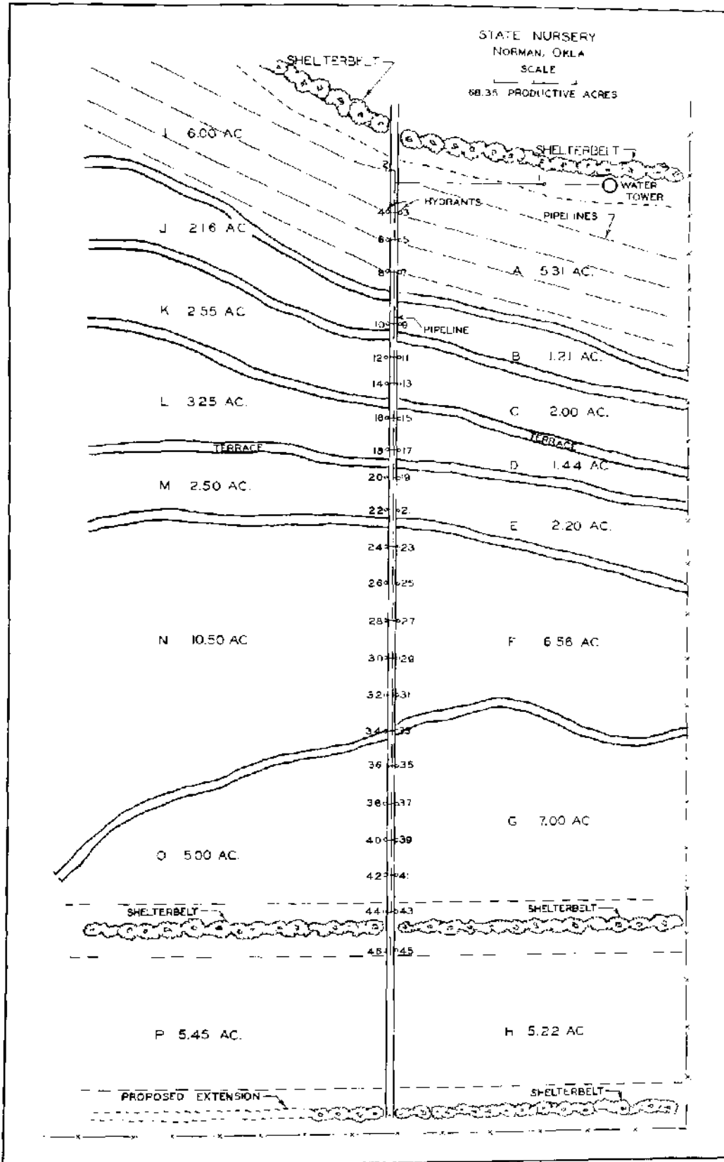
FIGURE 14. —Sprinkler irrigation system layout used at the Oklahoma State Nursery at Norman. Surface pipes of 4-inch diameter are laid on the contour between terraces from hydrants. The main pipeline is 8 inches in diameter.
