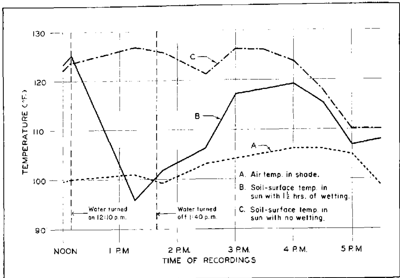
FIGURE 60.—Effect of watering on soil-surface temperatures A, Air temperatures in shade; B, soil-surface temperatures in sun with 1 1/2 hours of wetting; C, soil-surface temperatures in sun with no wetting. Towner Nursery, Towner, N. Dak.
