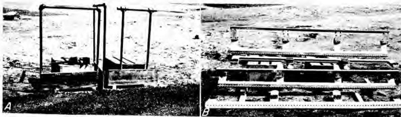
FIGURE 30.—Equipment for hand transplanting: A, Hand trenches formerly used at the Bessey Nursery; B details of the construction of an aluminum transplant board.
